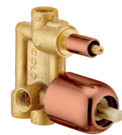
MR-34A | ₹-10154/- Single Lever Concealed Diverter Body (High-Flow) 4 Way
